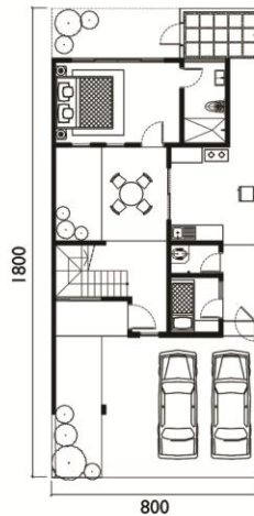
1 st floor
